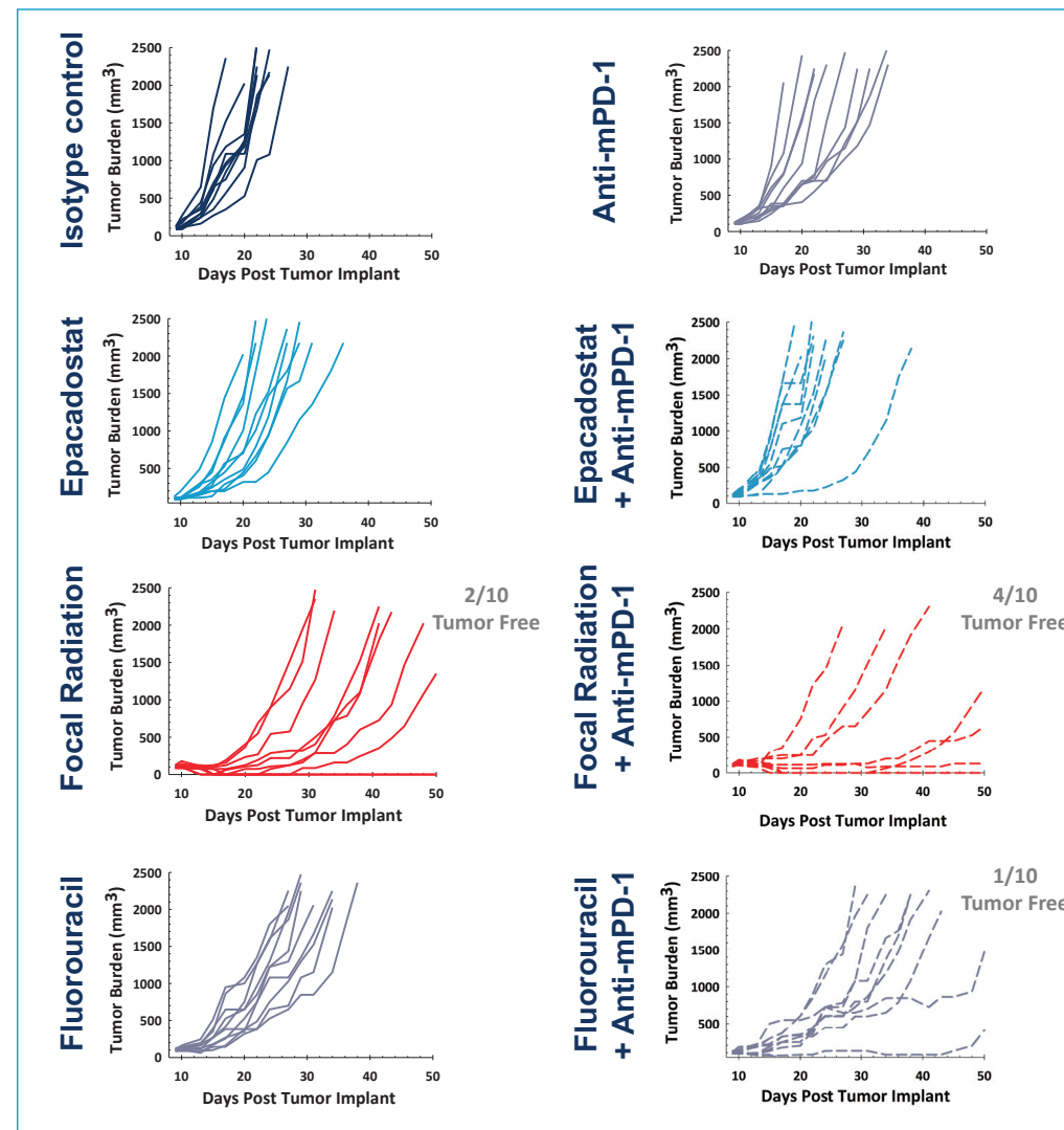
Figure 2. Efficacy evaluation of anti-mPD-1 combinations against CT26.
